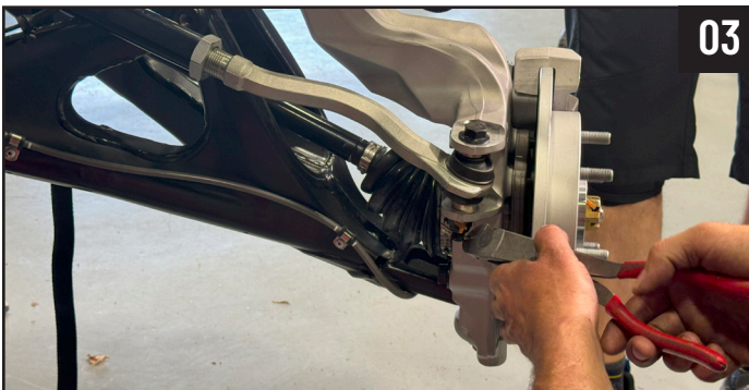
03 Loosen both inner and outer tie rod jam nuts. Mark the jam nut for correct alignment during re installation.
